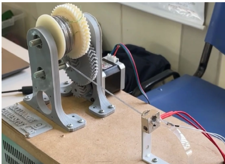
3D printer using filament made from PET bottles Source: courtesy photo
